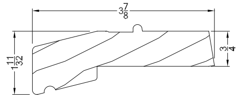
SS-H H Subsill
