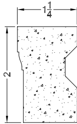
PVC-BM 2" PVC Brickmould
