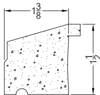
PVC-SN PVC Sill Nose
