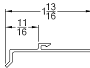
CSP Clad Sill Plate
